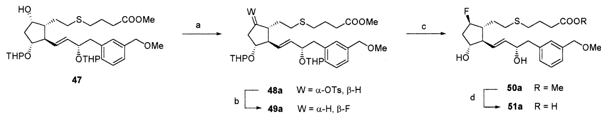
Scheme 8. Synthesis of 9 \beta -fluoro-5-thiaPGE 1 analogue 51a . Reagents: (a) p -TsCl, pyridine, DMAP; (b) TBAF, K 2 CO 3 , toluene; (c) p -TsOH, MeOH; (d) 1 N NaOH, MeOH.
