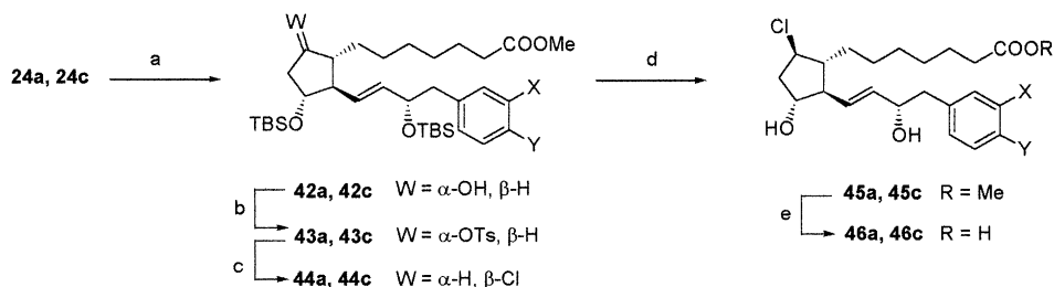
Scheme 7. Synthesis of 9 \beta -chloroPGE 1 analogues 46a and 46c . Reagents: (a) lithium tri- s -butylborohydride, THF; (b) p -TsCl, pyridine, DMAP; (c) TBACl, K 2 CO 3 , toluene; (d) p -TsOH, MeOH; (e) 1 N NaOH, MeOH.
