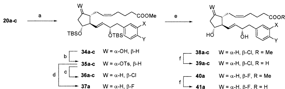
Scheme 6. Synthesis of 9 \beta -haloPGE 2 analogues 39a–c and 41a . Reagents: (a) lithium tri- s -butylborohydride, THF; (b) p -TsCl, pyridine, DMAP; (c) TBACl, K 2 CO 3 , toluene; (d) TBAF, K 2 CO 3 , toluene; (e) p -TsOH, MeOH; (f) 1 N NaOH, MeOH.
