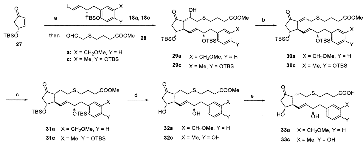
Scheme 5. Synthesis of 33a and 33c . Reagents: (a) 18a or 18c , t -BuLi, lithium (2-thienyl)cyanocuprate, ether, THF then 28 ; (b) MsCl, DMAP, CH 2 Cl 2 ; (c) n -Bu 3 SnH, (tBuO) 2 ; (d) (HF) n ·Py, pyridine, CH 3 CN; (e) PLE, EtOH, phosphate buffer.
