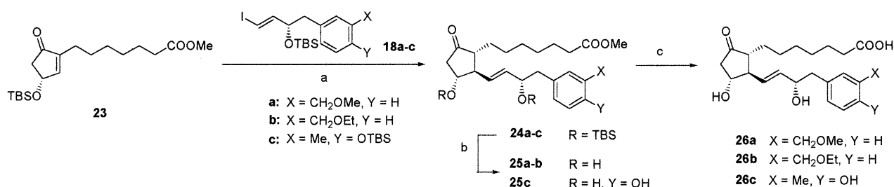
Scheme 4. Synthesis of 26a–c . Reagents: (a) 18a–c , t -BuLi, lithium (2-thienyl)cyanocuprate, ether, THF; (b) (HF) n ·Py, pyridine, CH 3 CN; (c) PLE, EtOH, phosphate buffer.
