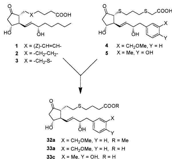
Scheme 1. Discovery of 16-phenyl- \omega -tetranor-5-thiaPGE 1 as highly selective EP4-receptor agonists 32a , 33a and 33c .
