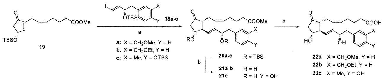
Scheme 3. Synthesis of 22a–c . Reagents: (a) 18a–c , t -BuLi, lithium (2-thienyl)cyanocuprate, ether, THF; (b) (HF) n -Py, pyridine, CH 3 CN; (c) PLE, EtOH, phosphate buffer.
